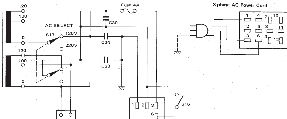
W Type Power Transformer (Y54-1290-61)
