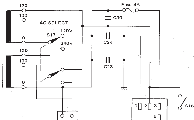
T Type Power Transformer (Y54-1290-51)
