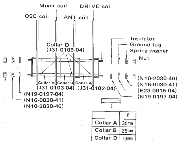
Fig. 12 Coil Pack Assembly
