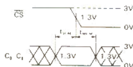
(5) Pulse delay timing
