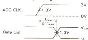
(5) Pulse delay timing
