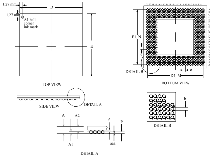
Figure 15 304-TBGA Drawing
