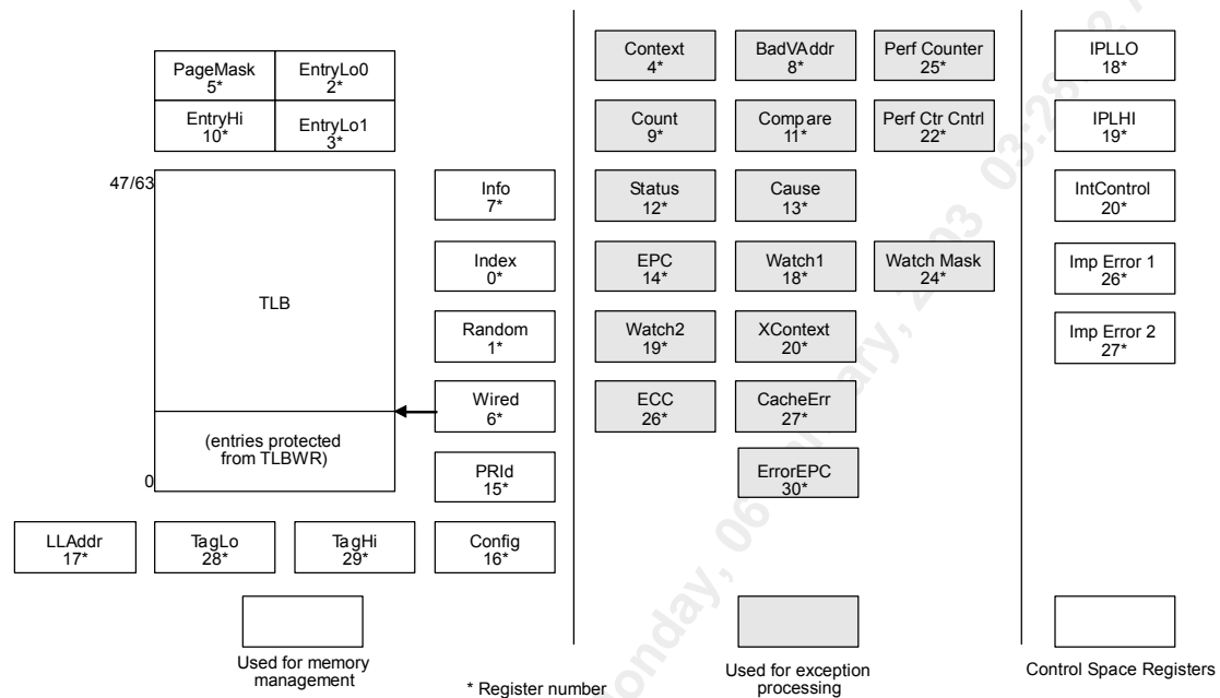
Figure 5 CP0 Registers
