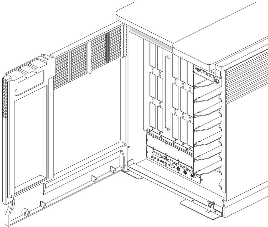
Figure 27 Eveready Chassis - Front Door Open
