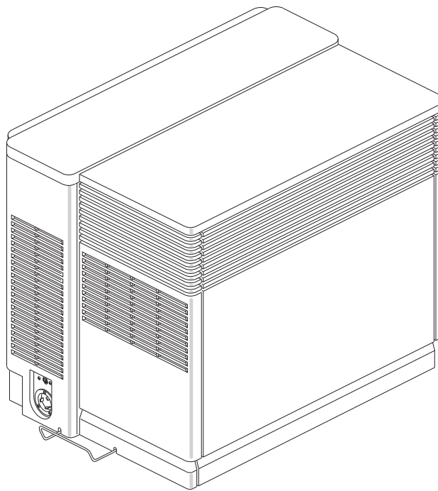
Figure 26 Eveready Chassis - Front & Rear Quarter Views
