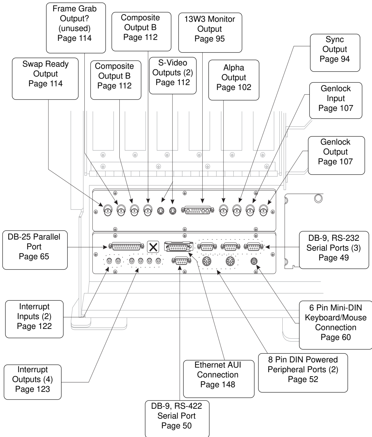
Figure 28 Eveready I/O Panel
