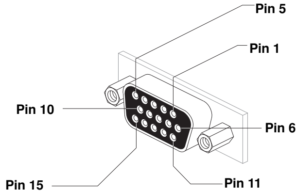
Figure 34 S-VGA Connector
