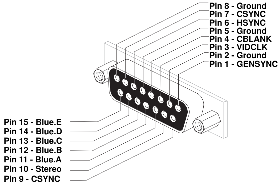
Figure 35 Genlock Option Connector
