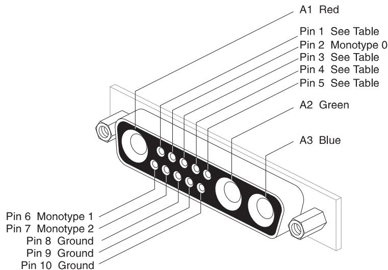
Figure 33 13W3 Monitor Output Connector
