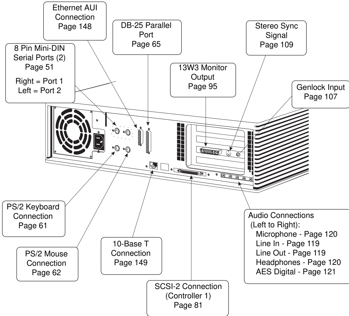
Figure 34 Indigo 2 I/O Panel
