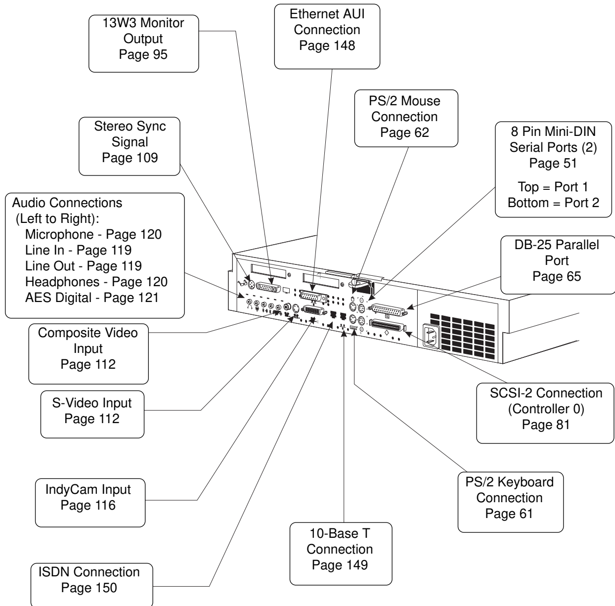
Figure 36 Indy I/O Panel
