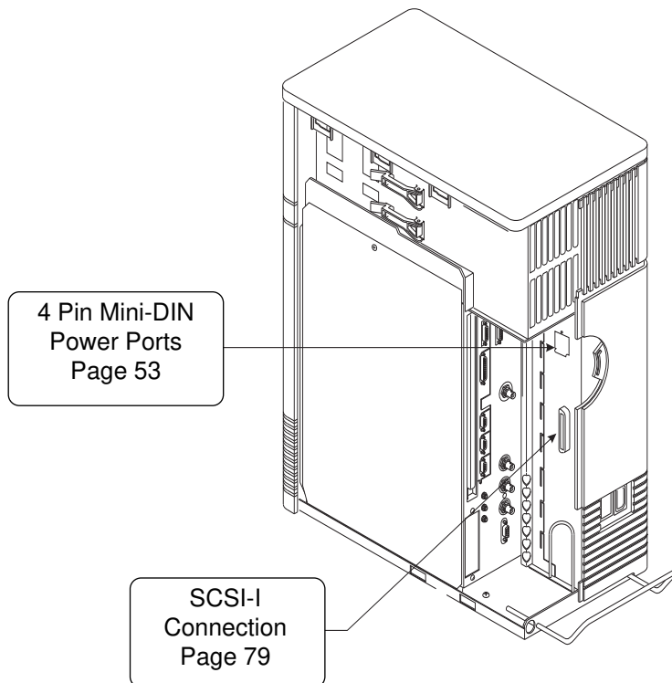
Figure 13 Personal IRIS Rear Quarter View Without Side Skin
