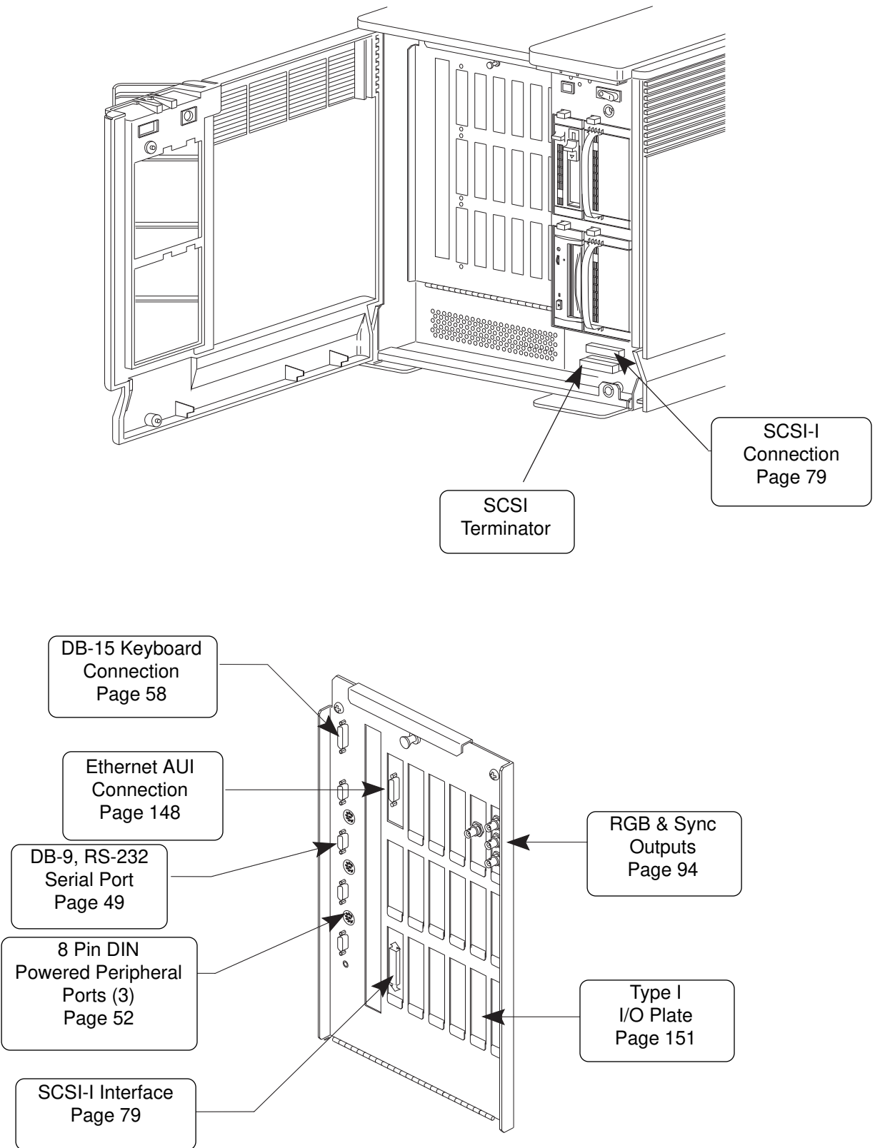
Figure 9 Diehard Front Drive Bays and I/O Panel
