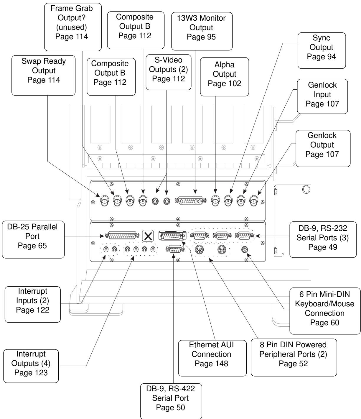
Figure 31 Terminator Rack I/O Panel
