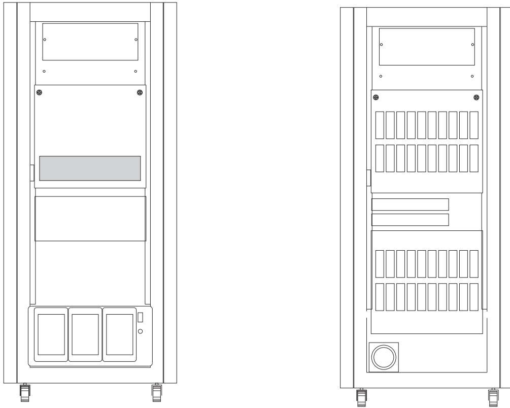
Figure 30 Terminator Rack - Front & Rear Views (without doors)
