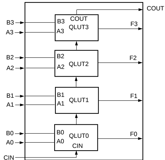
Figure 9. Ripple Mode
